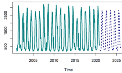
Forecasting of Surface_Pressure till 2025
