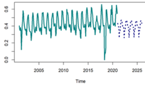
Forecasting of Specific_Humidity till 2025
